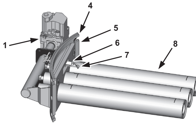
3-BURNER ASSEMBLY (for Input of 250 KBtu/H or higher)
