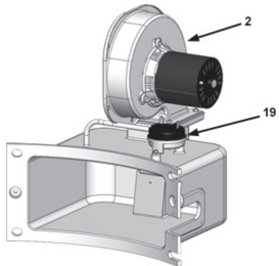
BLOWER ASSEMBLY
